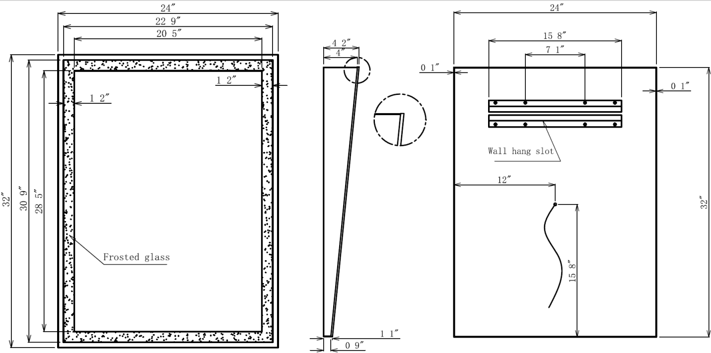
FRONT VIEW
