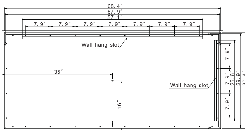
REAR VIEW
