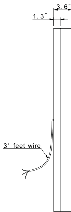
LEFT VIEW
