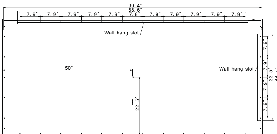
REAR VIEW
