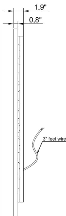
LEFT VIEW
