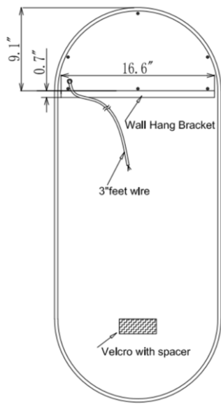
REAR VIE
