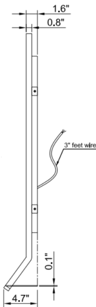
LEFT VIEW
