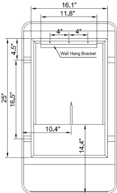
REAR VIEW
