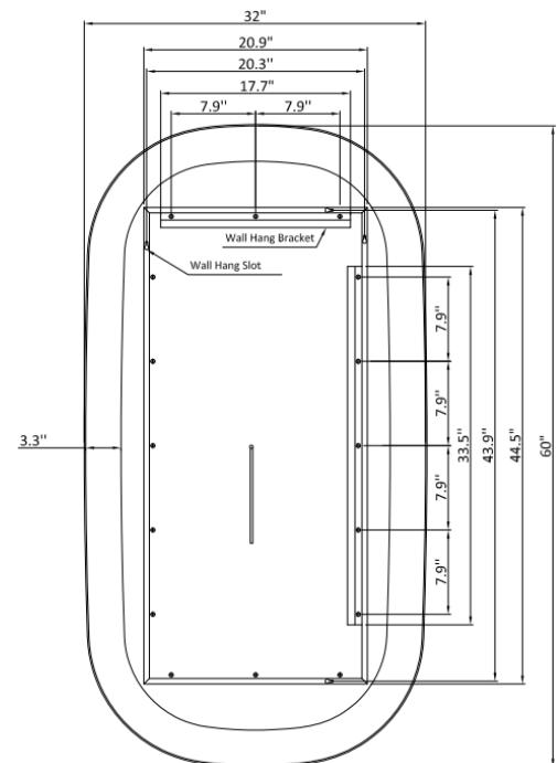
REAR VIEW
