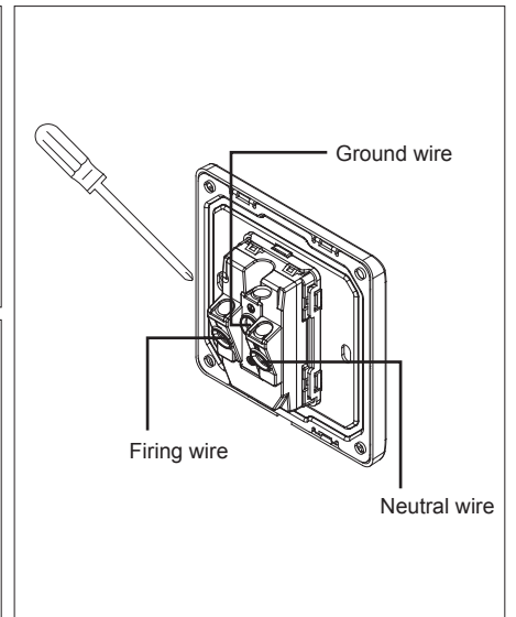
Step11. Connect the wiring with junction box.
