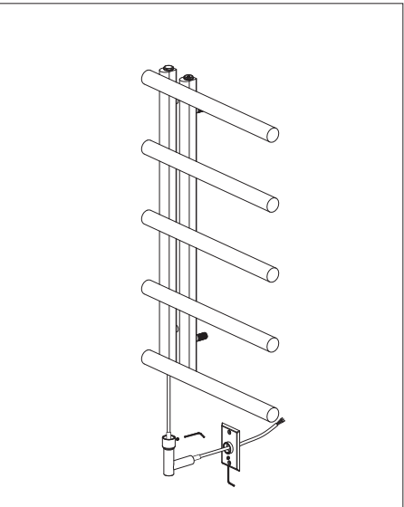
Step3. Get the electric wire through silicone hose and right angle decorative tube and then decorative cover. Tighten the tube and element first, then tighten the tube and decorative cover with allen wrench.
